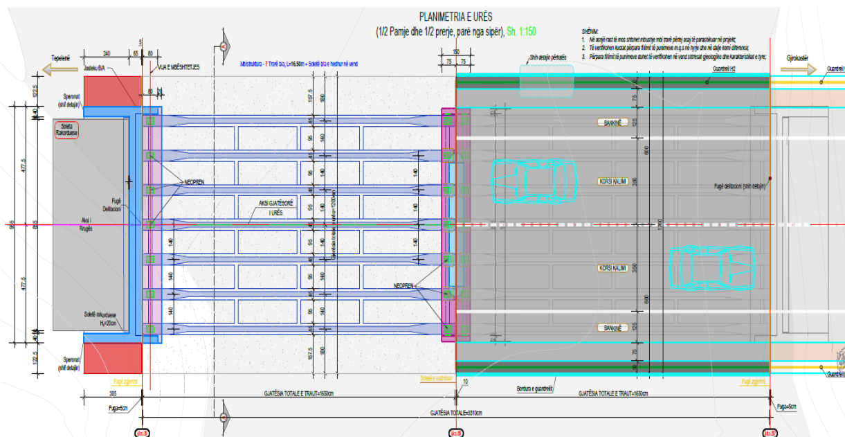
Figure 5. Top view of the new bridge
