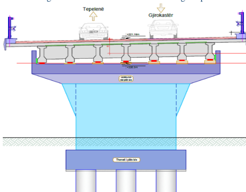
Figure 8. Cross section of the new bridge - pier
