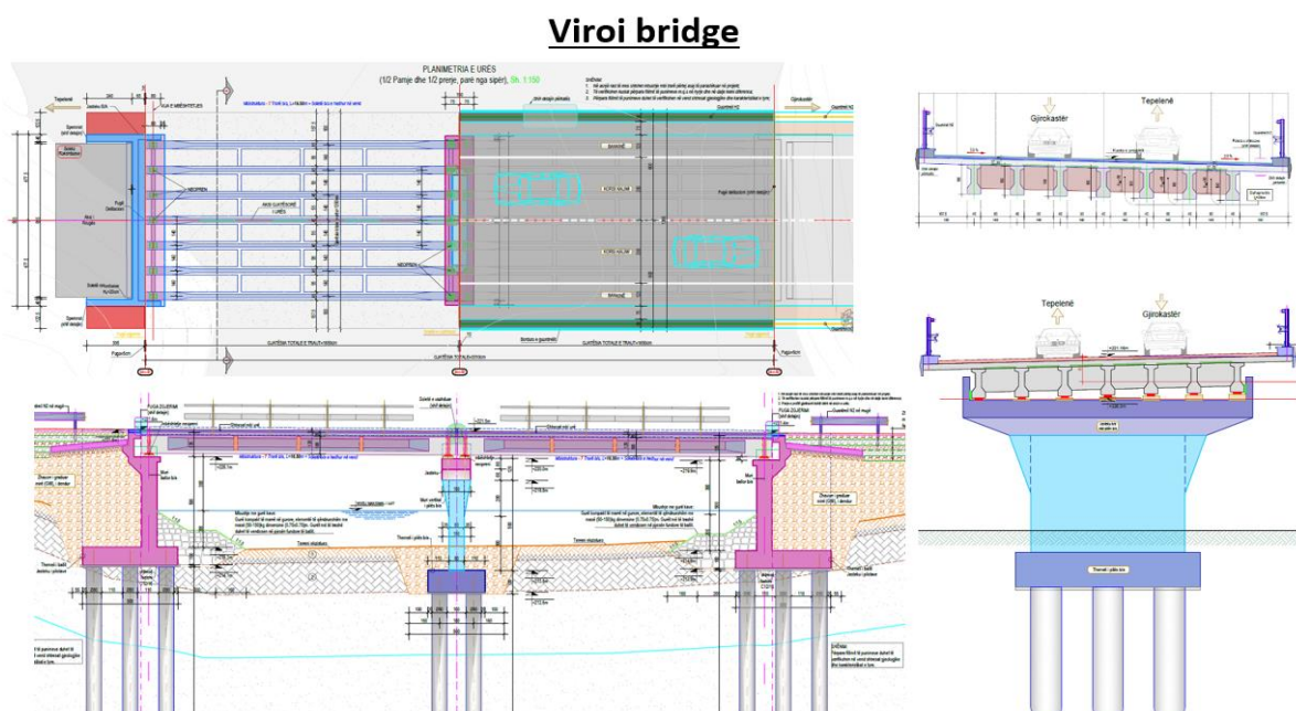
Figure 3: Technical design of Viroi Bridge
